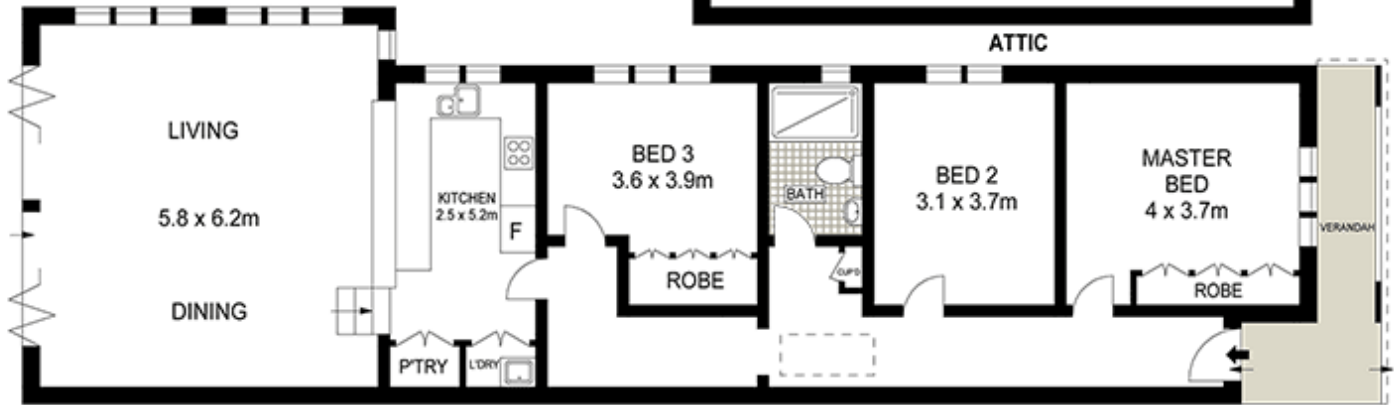
GROUND FLOOR
